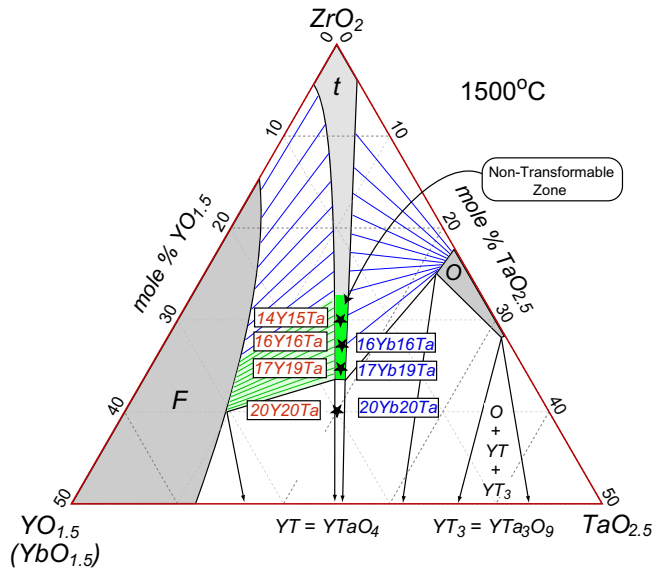
Fig. 1. Isothermal section of the \text{YO}_{1.5}\text{-TaO}_{2.5}\text{-ZrO}_2 ( \text{YbO}_{1.5}\text{-TaO}_{2.5}\text{-ZrO}_2 ) phase diagram at 1500 °C. The compositions studied are indicated with pentagrams. The compositional range of the “non-transformable zone” along the \text{ZrO}_2\text{-YTao}_4 quasi-binary is also indicated.
