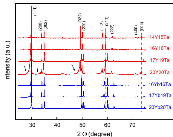
Fig. 2. X-ray diffraction patterns of the compositions studied. On the spectrum for the 20Y–20Ta sample, extra peaks on the shoulders of the peaks at 29.5^\circ , 33.9^\circ and 49.3^\circ were indicated by arrows and assigned to monoclinic \text{YTaO}_4 precipitated from the tetragonal major phase. Also indicated by dash lines are the consistent shifts of certain peaks with composition.
