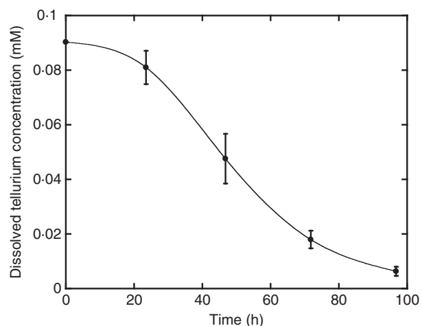
Figure 5 The change in soluble tellurium concentration over time during incubation with EPR3, as measured by ICP-MS. The points on the plot are the average of three replicates, and the error bars are the standard deviation of the three measured values. A cubic spline fit line is drawn through the points.
