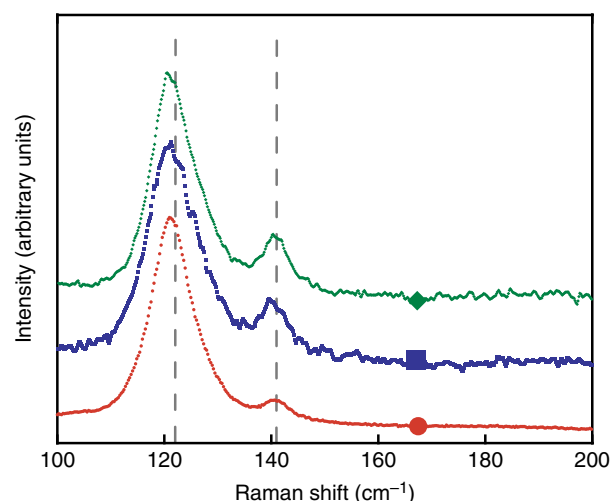
Figure 2 Raman spectra of EPR3 precipitations after incubation with tellurium dioxide, metallic tellurium and tellurite on solid media. Each precipitation exhibits Raman peaks distinctive of metallic tellurium, at 122 and 141 \text{ cm}^{-1} . These spectra were recorded from the boxed region shown in Fig. 4, suggesting that EPR3 is precipitating metallic tellurium away from the tellurium sources indicated. EPR3 precipitation—incubation with (◆) tellurium dioxide, (■) metallic tellurium and (●) tellurite.
