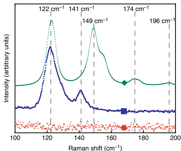
Figure 1 Raman spectra of standards of metallic tellurium, tellurium dioxide and tellurite (dissolved in solid artificial sea water (ASW) media) between 100 and 200 \text{cm}^{-1} . The metallic tellurium exhibits distinctive peaks at 122 and 141 \text{cm}^{-1} . The tellurium dioxide exhibits distinctive peaks at 122, 149, 174 and 196 \text{cm}^{-1} . The tellurite does not exhibit any Raman peaks. Standards of (◆) tellurium dioxide, (■) metallic tellurium and (●) tellurite.
