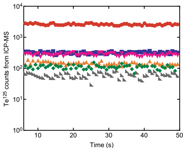
Figure 3 ICP-MS results for headspace sampling of tellurium 125 above EPR3. Samples of tellurite, metallic tellurium, tellurium dioxide, autoclave slime, bismuth telluride and cadmium telluride were incubated aerobically with EPR3 on solid artificial sea water (ASW) for 48 h. In the headspace of each sample, a gaseous tellurium species was detected. In controls of the tellurium compounds incubated on sterile solid ASW without EPR3, zero tellurium counts were detected during the sampling time, meaning no gaseous tellurium was detected. Gaseous tellurium from (●) tellurite, (▲) metallic tellurium, (◆) tellurium dioxide, (■) autoclave slime, (▼) bismuth telluride and (◄) cadmium telluride.
