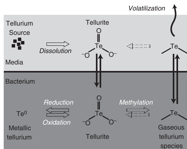
Figure 8 Schematic of proposed tellurium speciation in a bacterium and its media. Diffusion is represented by solid arrows, and chemical changes are represented by hollow arrows. We propose that a solid tellurium source (e.g. tellurium dioxide, autoclave slime, cadmium telluride and bismuth telluride) dissolves in the media to yield soluble tellurite. The tellurite crosses the cell wall, and the bacterium transforms it to either metallic tellurium or a gaseous tellurium species (for instance, dimethyl telluride by way of the Challenger mechanism). While there is undissolved tellurium source, the metallic tellurium–tellurite–volatile tellurium system is in steady state; solid tellurium dissolves to tellurite, which can be converted to a gaseous tellurium species, which escapes to the environment by volatilization. Volatile tellurium species may also be transforming back to tellurite (represented by dotted hollow arrow).
