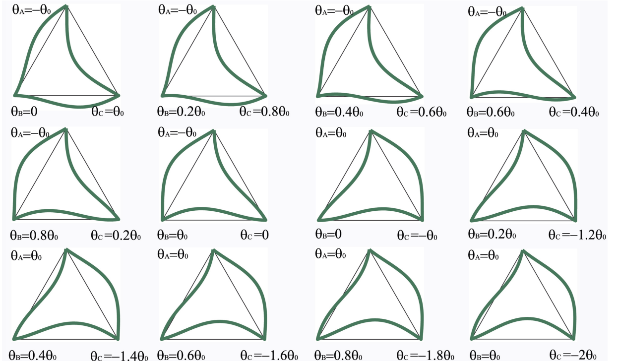
FIG. 3: Examples of critical eigenmodes. \theta_0 is used as reference angle.
