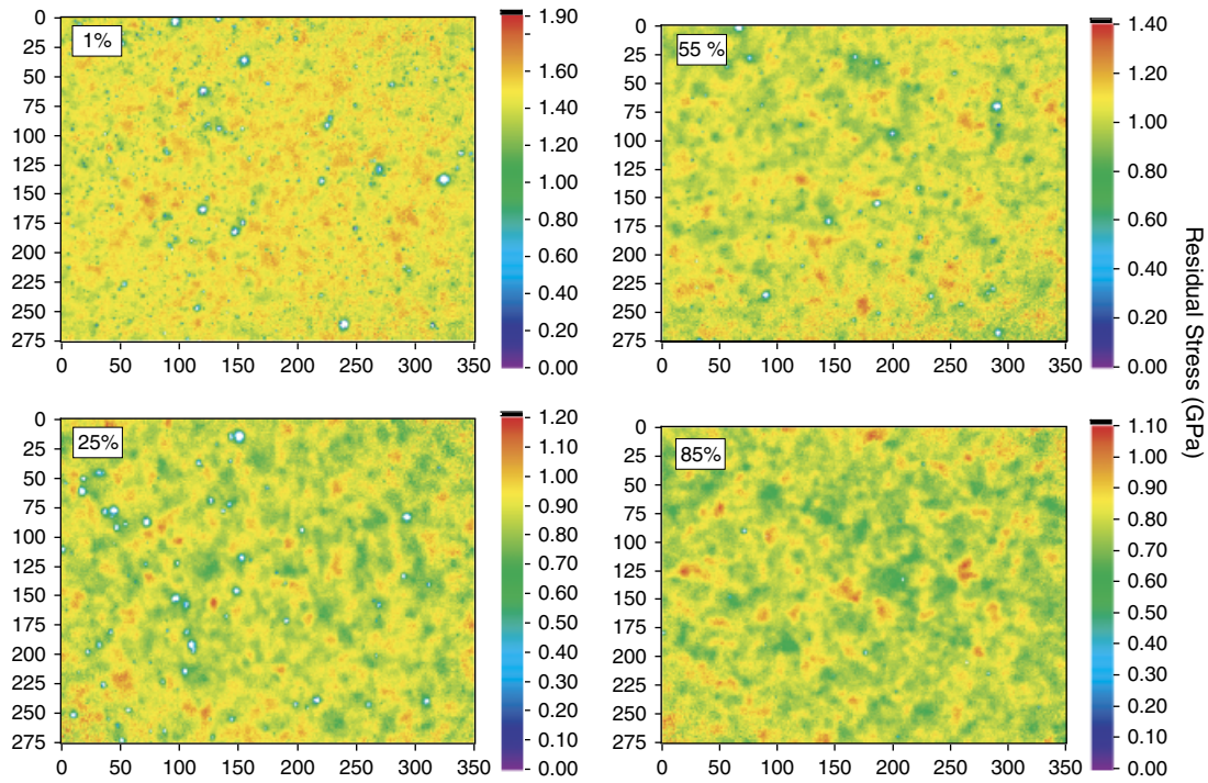
Fig. 6. Piezospectroscopic images of four coatings at different fractions of their average life. The color coding corresponds to the mean stress levels shown on the vertical color stripes on the right hand side of each panel. The numbers on the left hand ordinate and horizontal are pixels, each 16 \mu\text{m} in size, so the images correspond to areas of 4.4 \text{ mm} \times 5.6 \text{ mm} .
