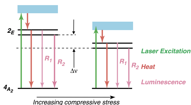
Fig. 4. Schematic of the energy levels of \text{Cr}^{3+} in alumina, the decay paths and the energy shift caused by a compressive stress.
