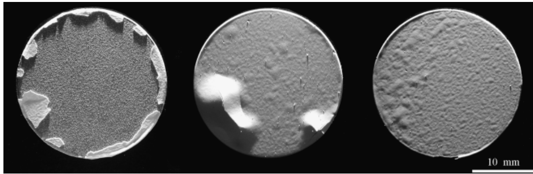
Fig. 1. Optical micrographs of EB-PVD deposited TBCs illustrating different stages in failure. Before macroscopic buckling (right), the formation of a macroscopic buckle (center) and after the TBC has everywhere spalled away except around the edges (left). The coated superalloy buttons are 25.4 mm (1 in.) in diameter.
