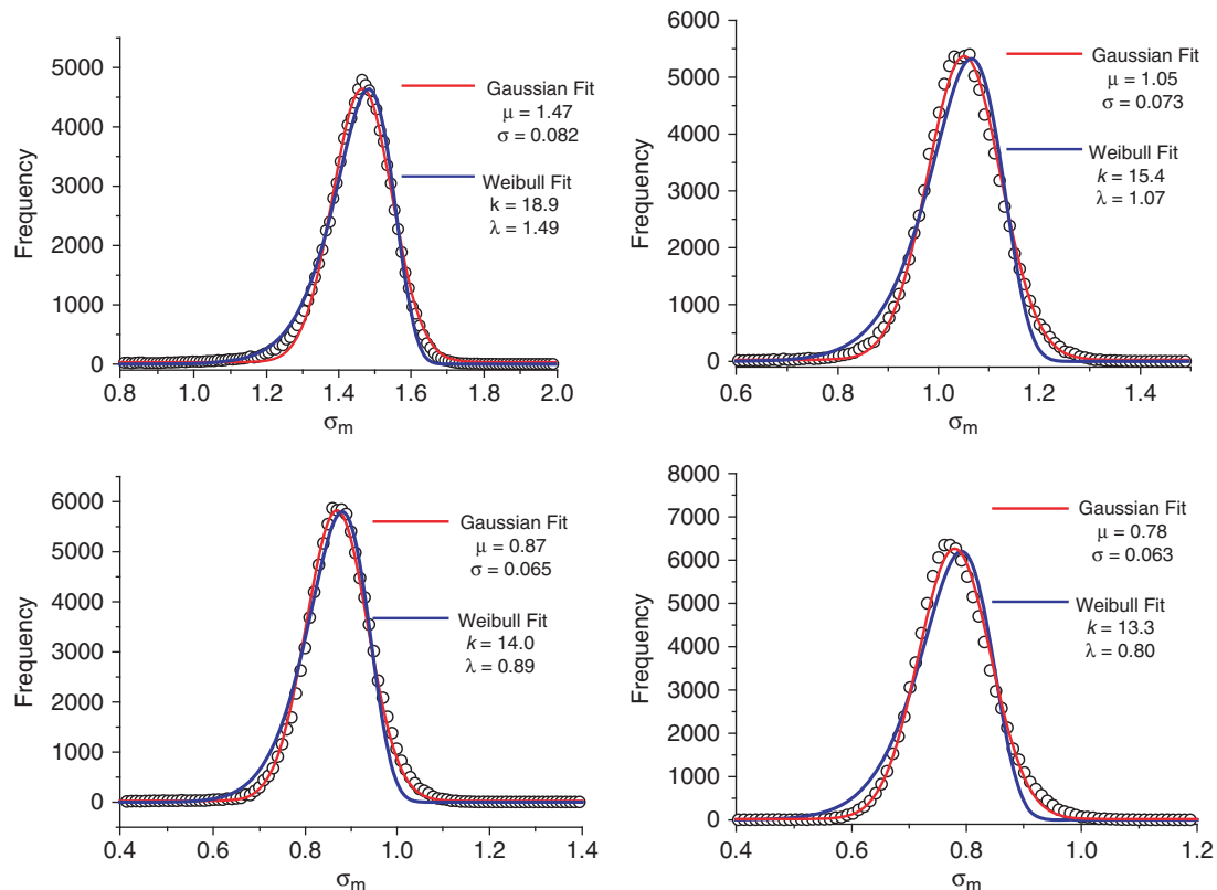
Fig. 7. Distribution functions of the stresses in the images shown in Fig. 6 as a function of the mean stress.
