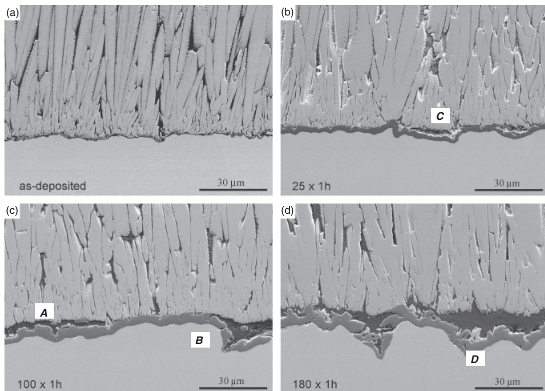
Fig. 2. Cross-sections of the alloy/TGO/TBC interfacial regions. (a) after deposition, and after (b) 25 (c) 100, and (d) 180 thermal cycles, each 1 h long, illustrating the thickening of the thermally grown oxide (TGO), the roughening of the interfaces, interface separations and the cracking of the TGO associated with the roughening. The TGO, which appears dark gray, is located between the columnar thermal barrier top-coat, above, and the aluminide bond-coated superalloy, below the TGO.
