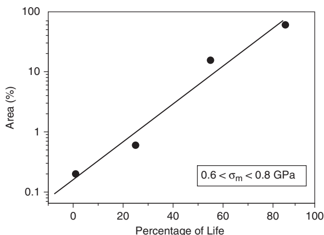
Fig. 9. Fractional area of the coatings where the mean stress lies in the interval 0.6–0.8 GPa as a function of the fractional life. Data obtained from the piezospectroscopic images in Fig. 6.
