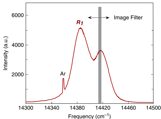
Fig. 3. Characteristic R-line luminescence from a TGO. The sharp line labeled Ar is from an argon discharge lamp used to calibrate frequency.
