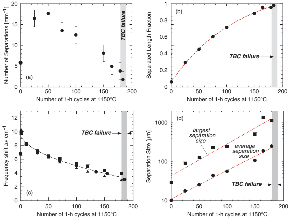
Fig. 10. Data obtained from analysis of SEM cross-sections. (a) Number density of separations, (b) proportion of the interface length that has separated, (c) piezospectroscopic shift, and (d) lateral size of interface separations, all as a function of the number of thermal cycles.
