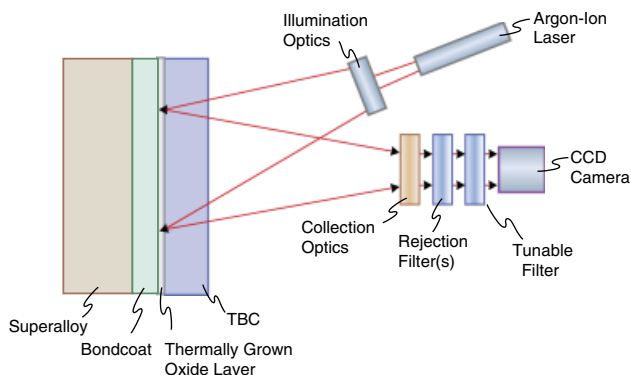
Fig. 5. Schematic of multispectral imaging system in which a TBC-coated sample is uniformly illuminated with an argon ion laser beam and the luminescence imaged onto a CCD through a variable wavelength tunable Fabry–Perot filter.
