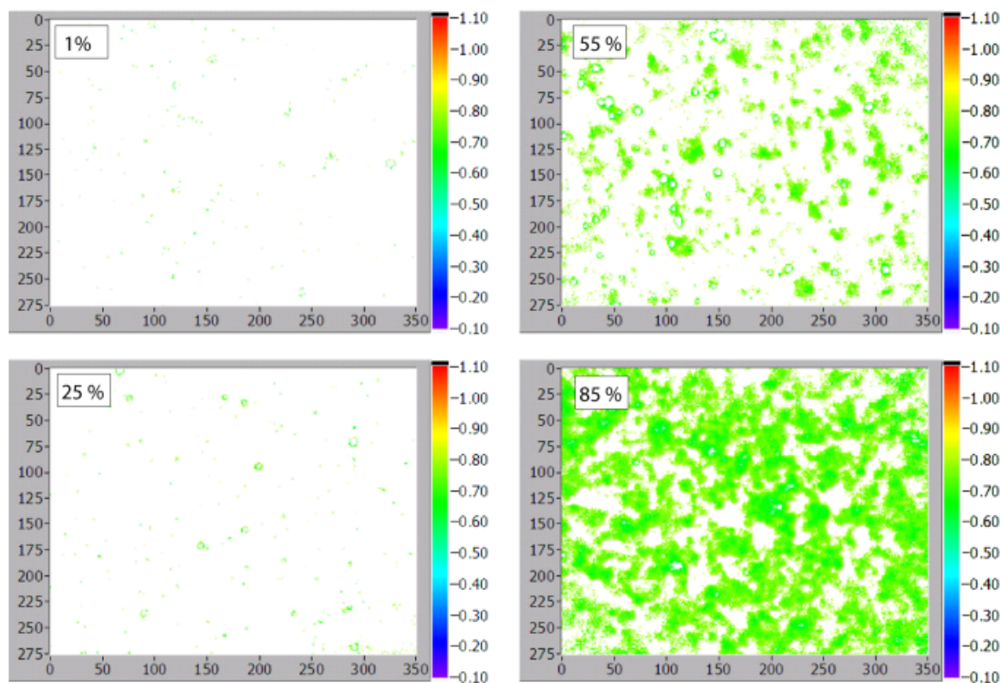
Fig. 8. Filtered piezospectroscopic images of Fig. 6 showing in green those regions where the mean stress in the thermally grown oxide is between 0.6 and 0.8 GPa. The white regions correspond to regions where the local mean stress is above 0.8 GPa. The numbers on the left hand ordinate and horizontal are pixels, each 16 \mu\text{m} in size.
