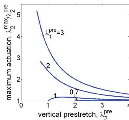
Fig. 6 Maximum actuation of a fiber-constrained membrane. The maximum actuation \lambda_2^{\max}/\lambda_2^{\text{pre}} is plotted as a function of the vertical prestretch \lambda_2^{\text{pre}} for several values of the horizontal prestretch \lambda_1^{\text{pre}} .
