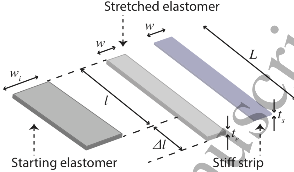
Figure 2. Geometric parameters for the elastomer and stiff strip. The elastomer strip starts in a relaxed state (left), then is stretched uniaxially (middle) by a strain of s = \Delta l/l to match the length ( L ) and width ( w ) of the stiff strip (right).
