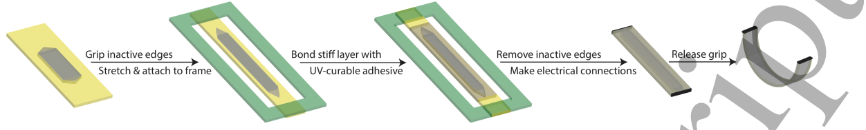
Figure 4. Fabrication of pre-stretched structure. The multilayer elastomer actuator starts in a relaxed state. We grip the inactive edges and apply the desired strain level to the elastomer. With the elastomer still in the strained state we apply uncured adhesive and a stiff strip to one side of the elastomer. After curing the adhesive, the grips are removed and the inactive sections are cut which leads to a curved elastomer-strip minimum energy structure.
