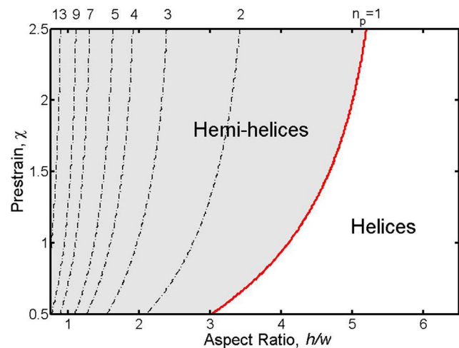
Figure 8. Contour plots showing the value of n for which the growth rate is maximum as function to \chi and h/w . The growth rates are calculated for P = 0.981P_{cr} . Black dotted lines show the boundaries between modes with different number of perversions n_p , while the red line corresponds to n_p = 1 and separates hemihelices (on its left) from helices (on its right). For clarity not all the higher modes are shown. doi:10.1371/journal.pone.0093183.g008
